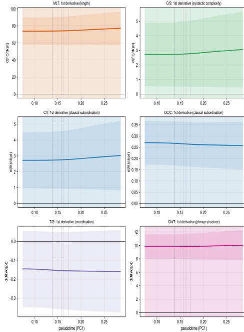
Figure 2. First Derivatives of GAM-Fitted Curves with 95% Simultaneous Confidence Bands
