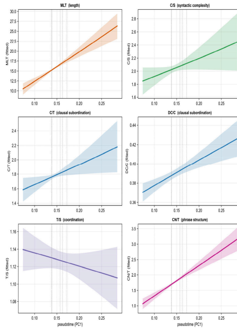
Figure 1. GAM-Fitted Curves of Six Syntactic Complexity Indices along Pseudotime
